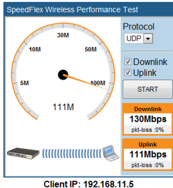
FIGURE 250 When the test is complete, the tool shows the uplink and downlink throughput and packet loss percentage
